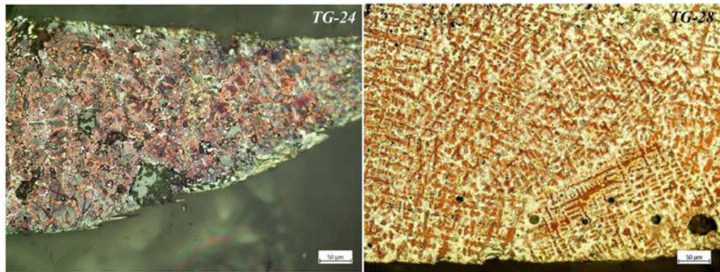
Fig. 10: Metallography of samples TG-24 and TG-28 shows dendritic microstructures indicative of casting (Authors, 2024).
